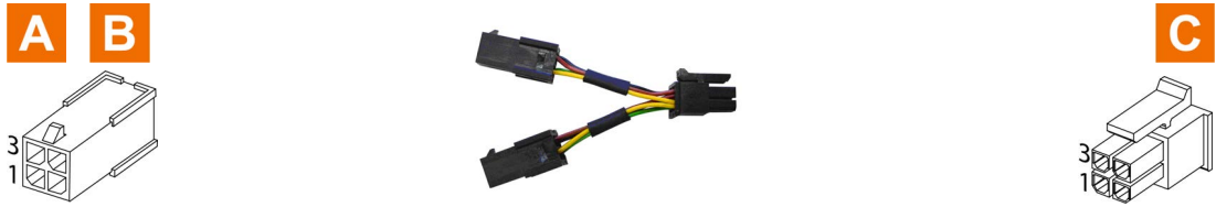
Figure 3-10 CAN-Y Cable
