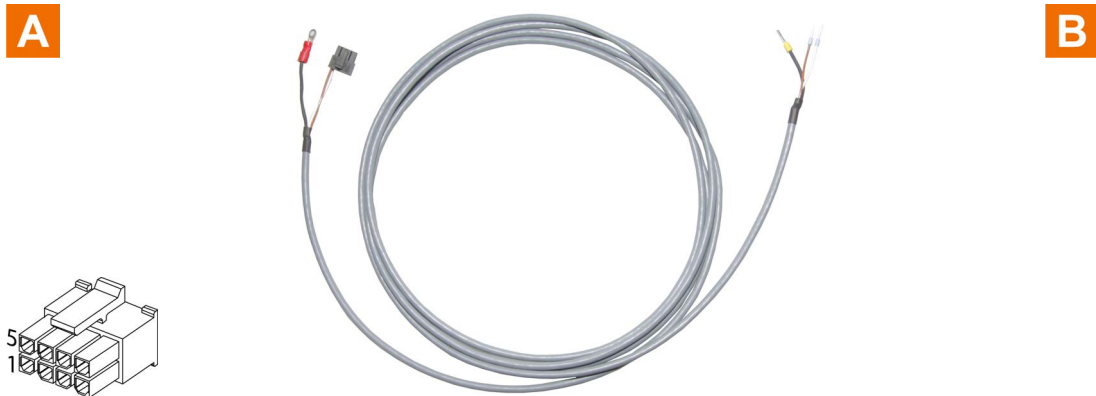
Figure 3-5 Motor/Hall Sensor Cable
